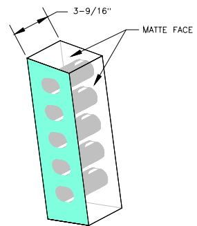
3D VIEW
