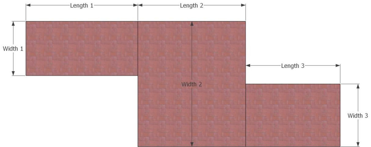
Patio Calculation Diagram
